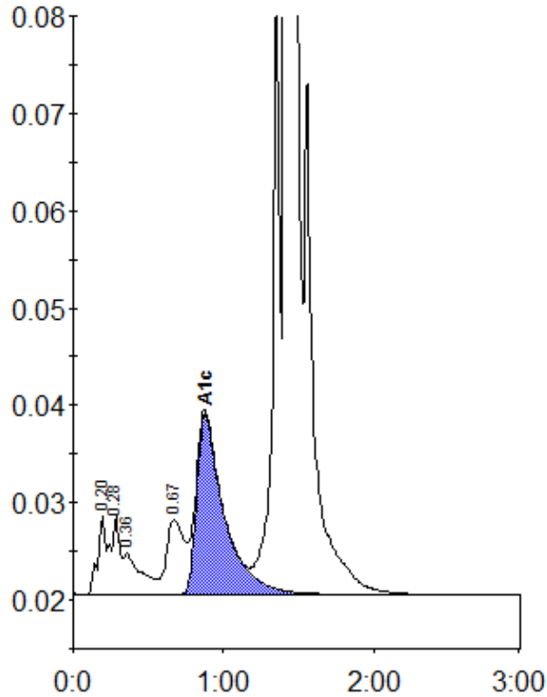
Peak table - ID: 10454232
